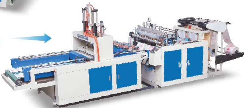
双线热切背心袋制袋机 Double lines hot cutting T-shirt bag making machine
