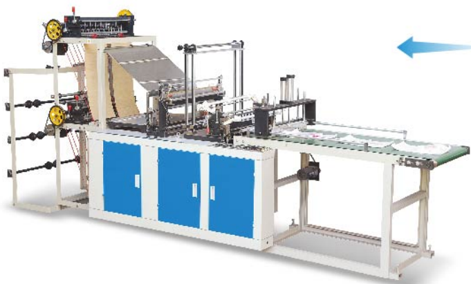
冷切制袋机带输送带 Cold-cutting bag making machine with conveyor
